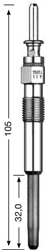
Y-507 J M 10 x 1.0 10 Hex 11 V DP 32
