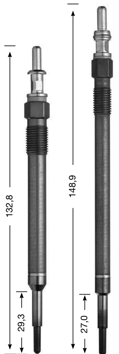
CZ 106 M 10 x 1.0 10 Hex 7 V DP 53
