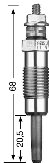
Y-935 U M 12 x 1.25 12 Hex 11 V DP 23
