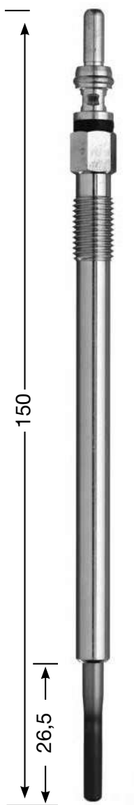
Y-8002 AS M 8 x 1.0 8 Hex 4,4 V DP 51
